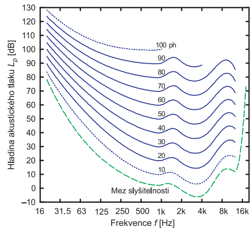
Obr. I.2.3 : Křivky hladin stejné hlasitosti. Adaptováno z Y. Suzuki et al: Precise and Full-range Determination of Two-dimensional Equal Loudness Contours , Research Institute of Electrical Communication, Tohoku University, Japan (2003).
